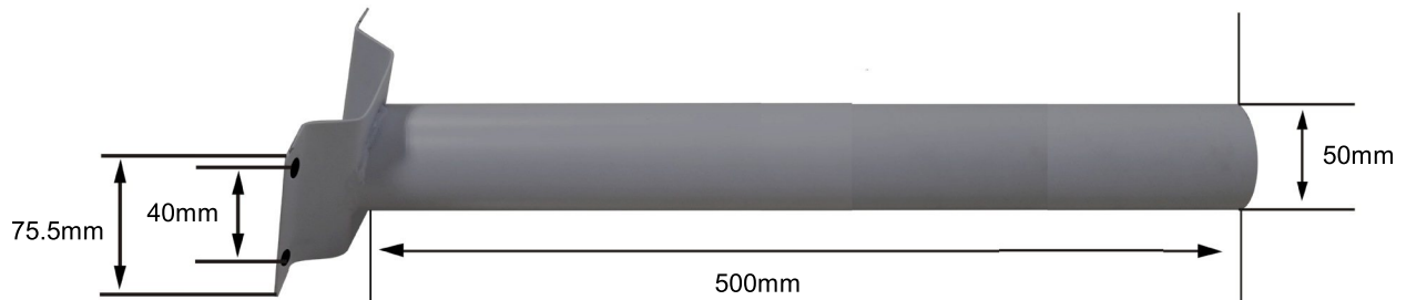
Arm bracket, Model: P50050-1
